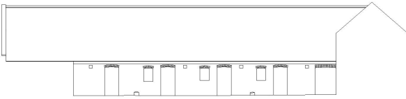
SECTION CC
